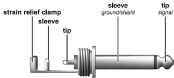
Fig .4.4: 1/4" TS connector
